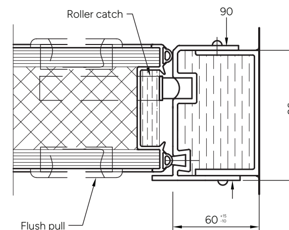
Horizontal Section - Wall Jambs
