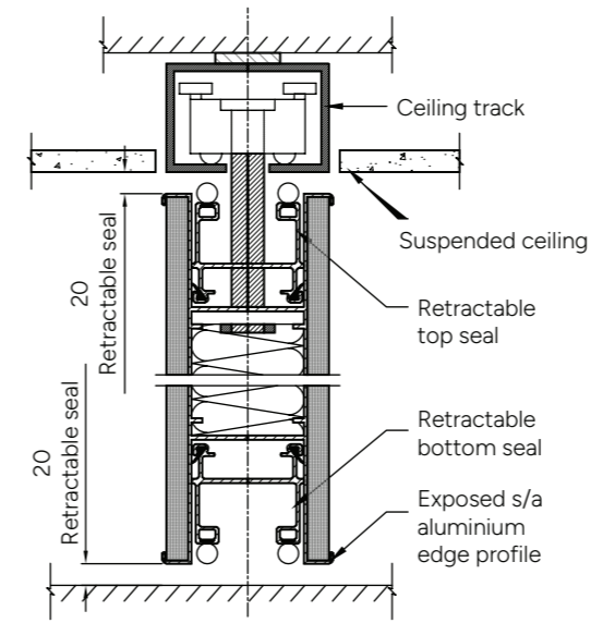
Vertical Section Through Standard Panel
